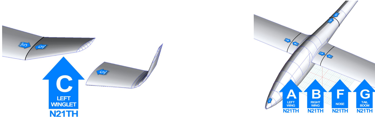
Sailplane Full Cover Set Graphic Indicators (Discus 2B, 3D model)
