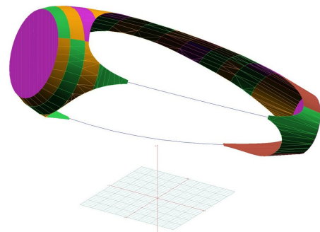
Falcon 6X Engine Cover, 3-Strap Type
