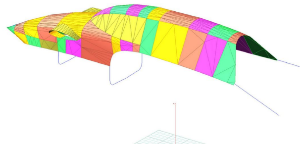
Cozy Classic Canopy/Nose Cover, 3D model
